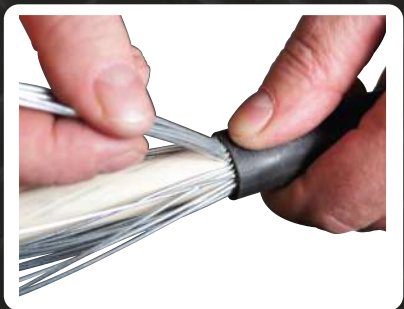
STEP 3: REMOVE OUTER SHEATH
