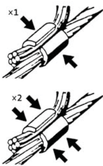
Crimp sequence.
