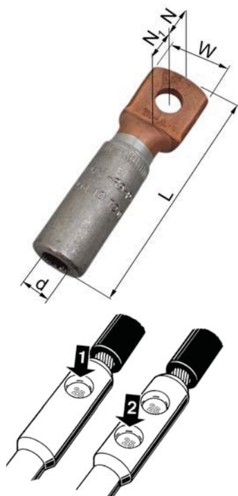
Crimp sequence.
