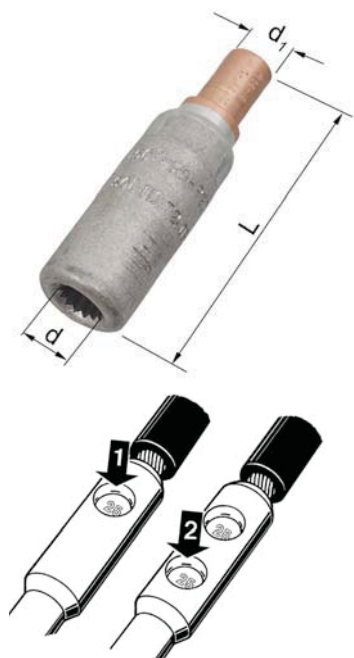
Crimp sequence.
