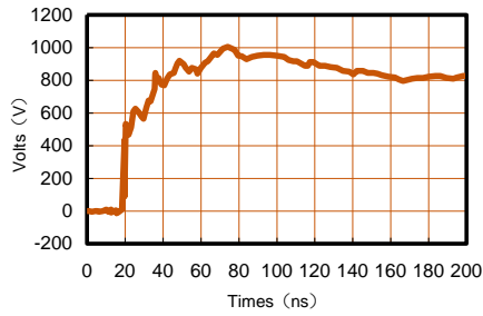
Original ESD waveform at 1 kV
