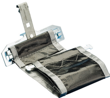
nVent CADDY Cat 425 Adjustable Cable Support with C Purlin Clip
