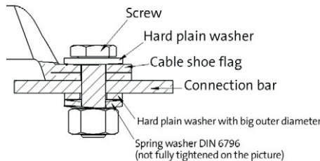
Bolt joint with spring washer.
