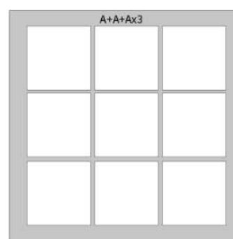
A+A+A x 3 (9 openings, 3 in a row x 3 high 120x120mm)
