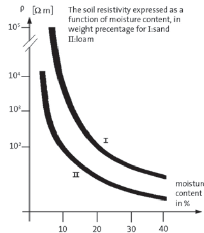
Soil resistance in relation to humidity.
