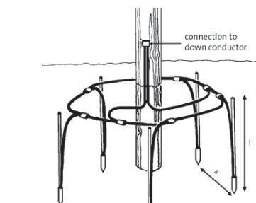
Parallel connection.
