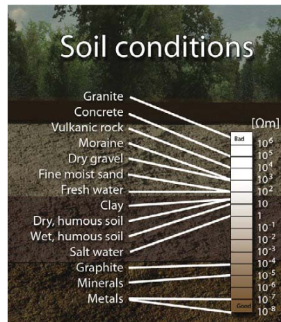
Resistivity in different soil conditions.
