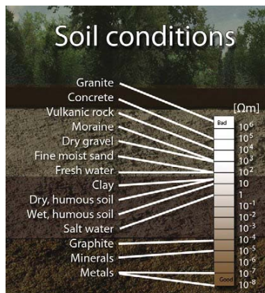
1. Resistivity in different soil conditions.
