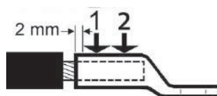
Crimp sequence for two crimps.
