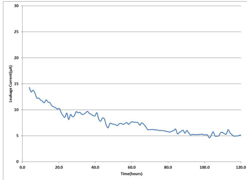
Fig 10: Leakage Current
