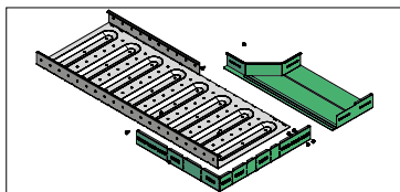
Fixed branching piece 90° right with coupling/reducer CSU089600xx
