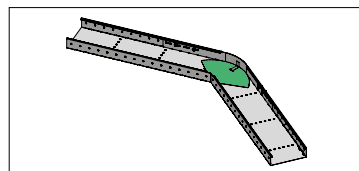
Place the Fixed adjustable bend on the inside of the cable tray.
