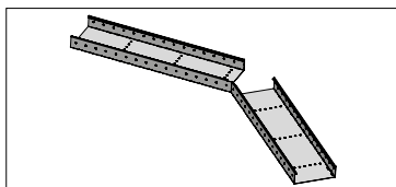
Make a V-shaped cutout at the bend
