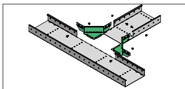
T-connection with 2 pieces CSU361100x2
